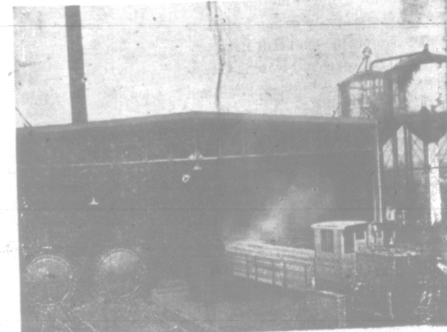
Into one of four retorts at Union Pacific's tie-treating plant at The Dalles, Ore., goes a 16-tram train of 300 crossties for a 22 hour bath in hot creosote petroleum which will greatly increase the ties' resistance to decay and extend by many years their service life.
