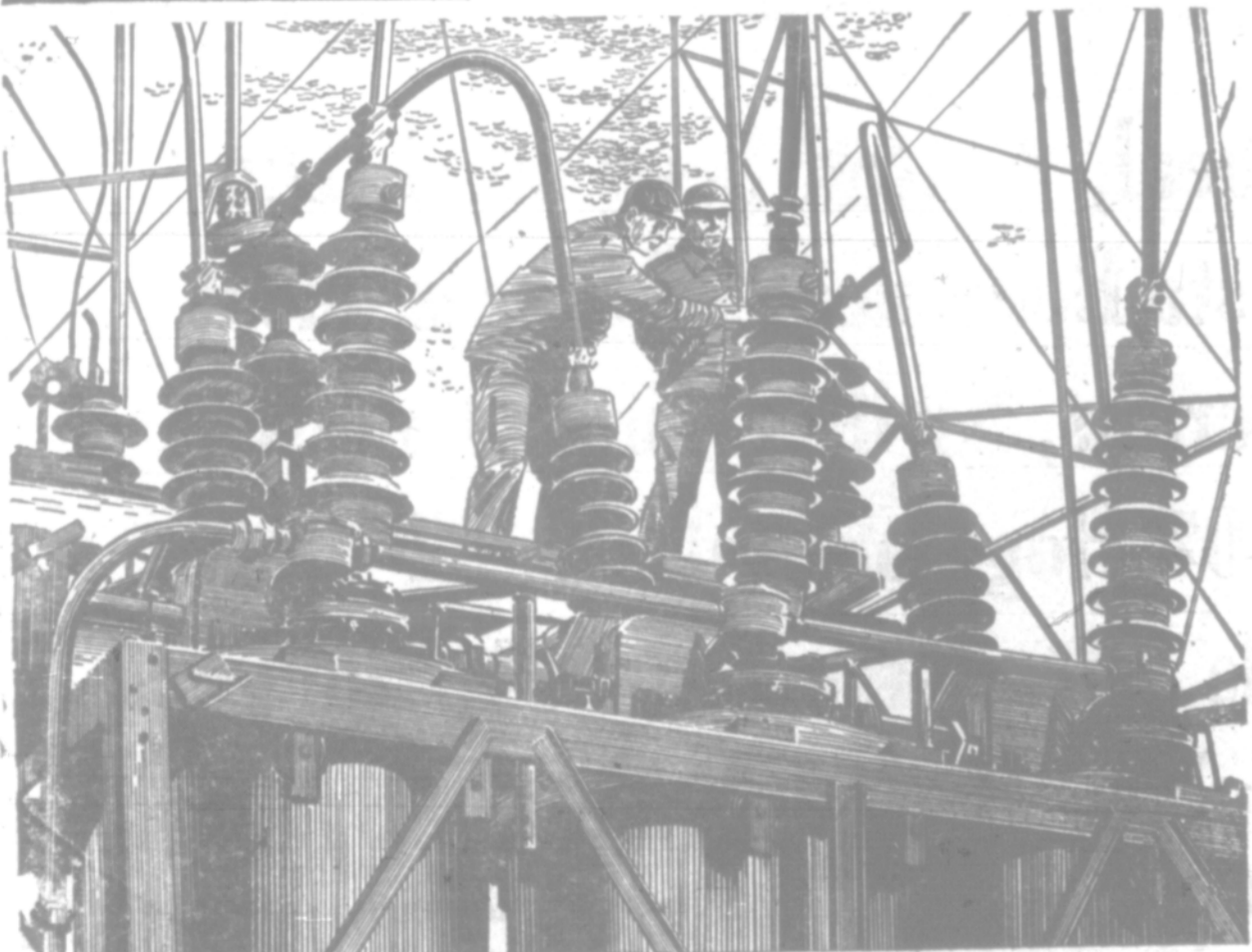
MORE CIRCUIT-BREAKERS costing about $20,000 each are being installed this year on the PP&L system. They are "fuses" to isolate trouble areas and improve efficiency of the Northwest Power Pool. PP&L is a pioneer partner in the Power Pool, which ties together the 300 public and private power plants of the Pacific Northwest.
