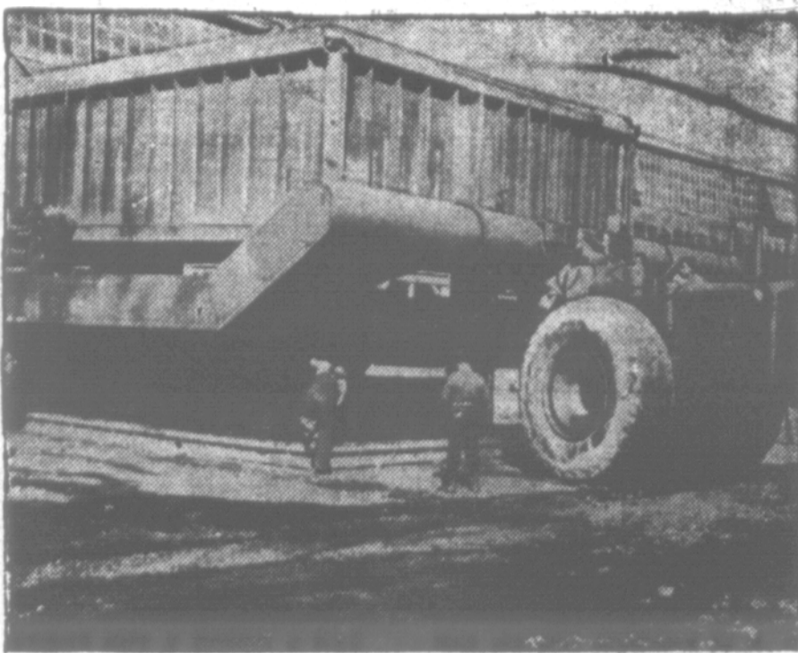
URNS OUT A HOUSE A DAY . . . New machine developed by E. G. LeTourneau, Peoria, Ill., will turn out a house with two bedrooms in 24 hours. The machine can be rolled into position on a home site on pneumatic tired wheels, pour the concrete and move on to the next site within 24 hours. The mass production idea has been demonstrated to Wilson W. Wyatt, FHA. Unions are expected to object to this type of construction.
