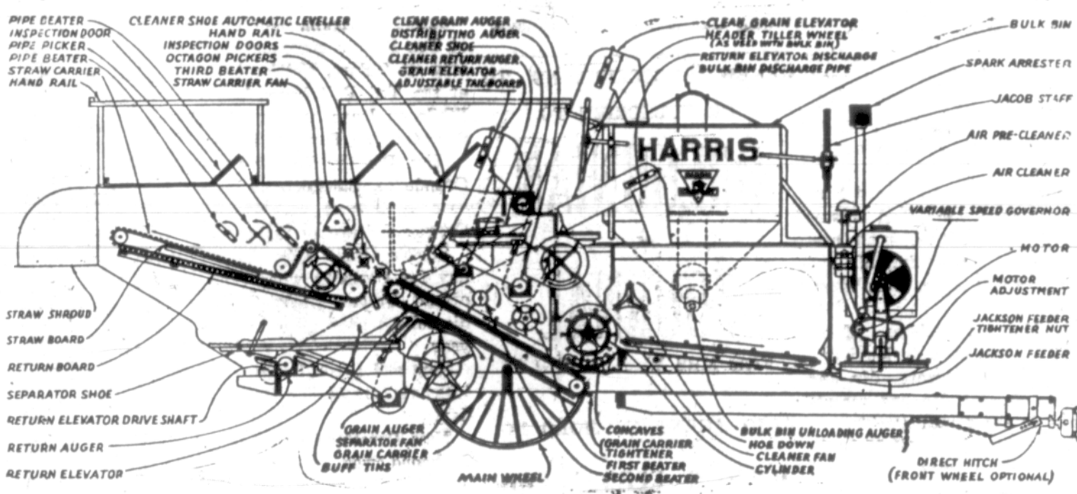
Typical Cross Section Harris 30-38 1944 Model
