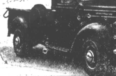
Pick-Up bodies available in 76, 88 and 102 inches (inside body) lengths on 115, 125, and 136-inch wheelbases.
