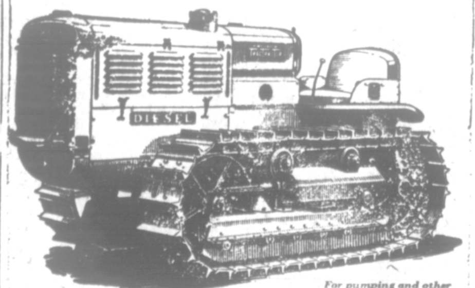
For pumping and other heavy-duty stationary work a McCormick-Deering Diesel Power Unit is available.
