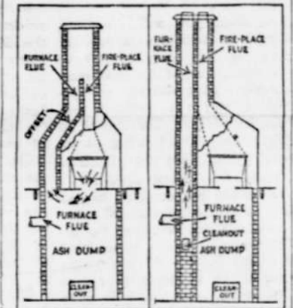
(Left) Furnace Flue Offset for Fire place. (Right) Correct Double Flue.
