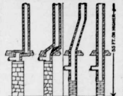
Two Examples of Bad Offsets; One, of Less Undesirable Slope. At the Right, an Ideal Chimney.
