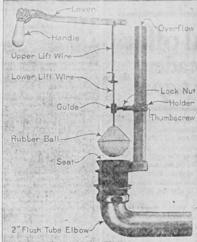
Flush Valve and How to Repair It.
