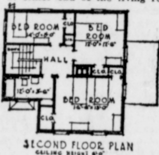
SECOND FLOOR PLAN Ceilings 8'0" to 8'6" © Celotex Institute, Chicago, 1926.
