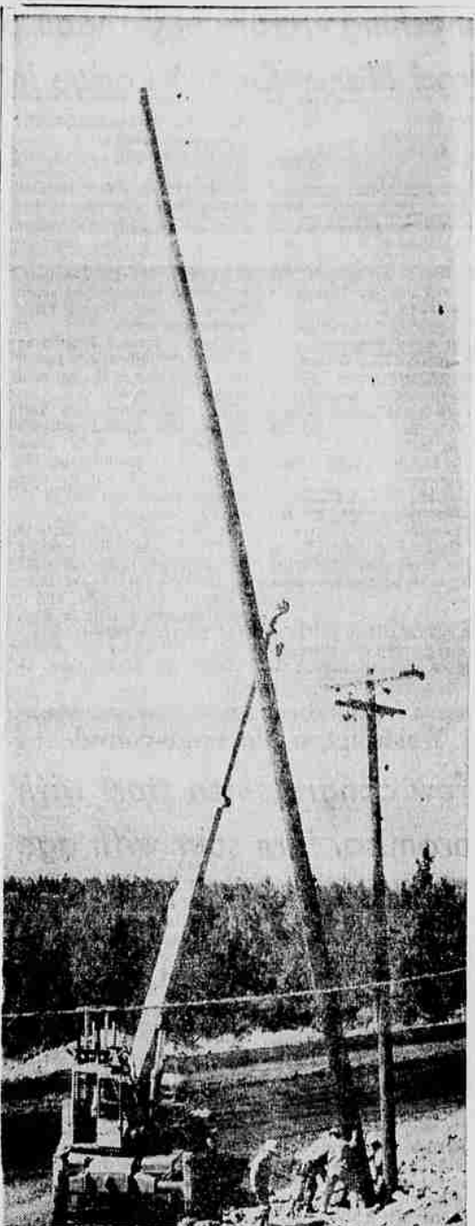
GIANT POLE ERECTED — Erecting new power pole for the Pacific Power & Light Company system serving Bend resulted in the above dramatic photograph of an 80-foot giant being set by construction crew straining at the base of the big timber. Pole will carry both 69,000-volt transmission line and 12,500-volt distribution circuit.
