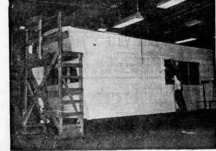
TOP: Bridge-steel I-beams, all electrically welded, form the rugged, pre-membered chassis for each coach. CENTER: Heavy fiberglass insulation in walls and ceilings provide important "hidden" quality feature. BELOW: Gleaming, pre-painted aluminum panels and trim complete another Imperial Mobile Home.
