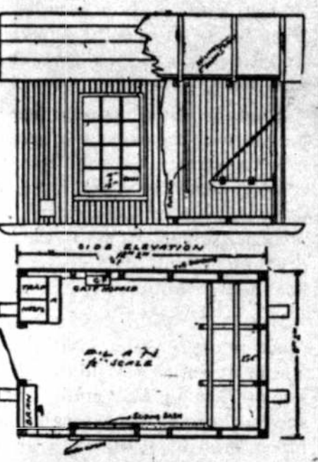
PLAN OF INTERIOR.
