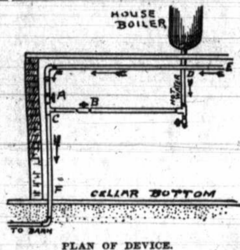
PLAN OF DEVICE.
