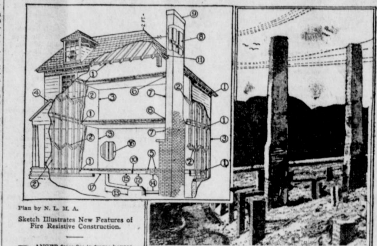
Plan by N. L. M. A. Sketch Illustrates New Features of Fire Resistant Construction.
