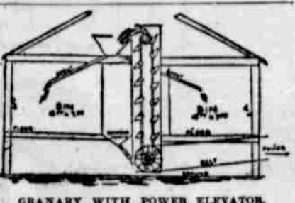
GRANARY WITH POWER ELEVATOR.
