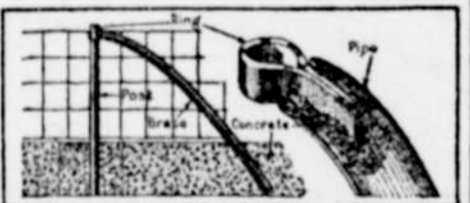
Iron Pipe Post Brace.
