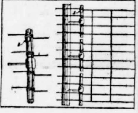
Wire Stretcher.
