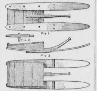
Runners Made of Barrel Staves.
