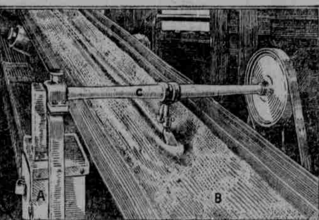
This device takes a test sample for the chemist every 8 seconds. "B" is the cement on a moving belt, leaving the grinding mill. "C" is a revolving hollow shaft. As the dipper picks up a bit of the flour-like material it is carried through the shaft "C" and deposited in the locked box "A".
