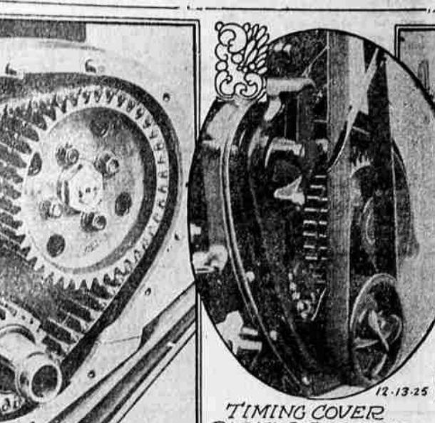
TIMING COVER PARTLY CUT AWAY TO SHOW TIMING CHAIN
