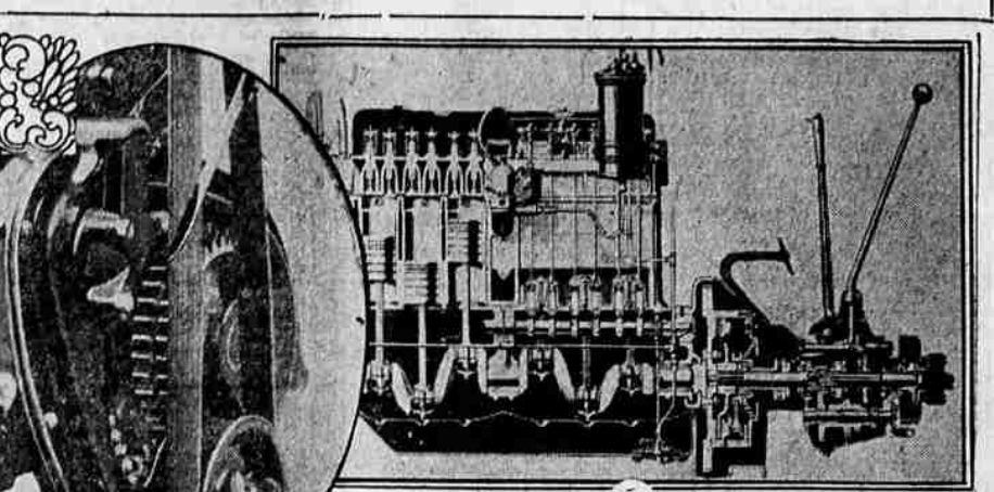
SIDE VIEW OF OVERHEAD VALVE ENGINE SHOWING TIMING CHAIN AT FRONT
