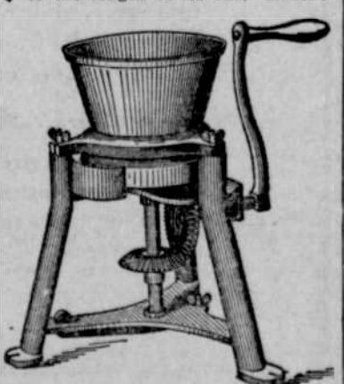
A Hand-power Paint Mill.
