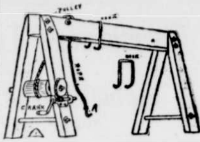
BUTCHERING DEVICE.
