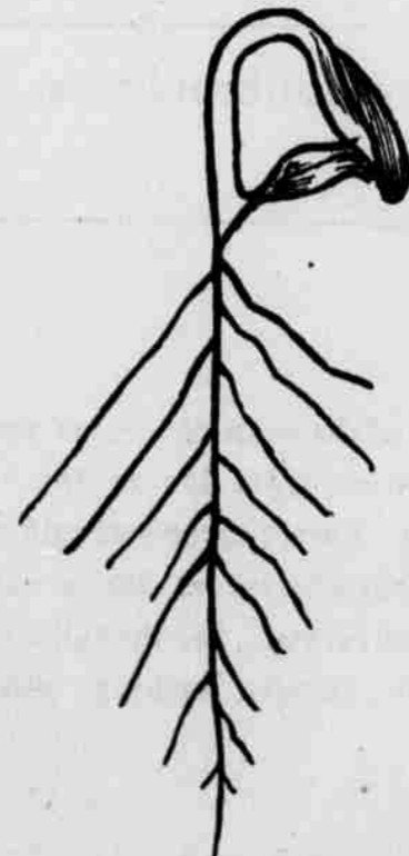
FIG. 2.—HOW A SQUASH PLANT TAKES OFF ITS SEED COAT.
