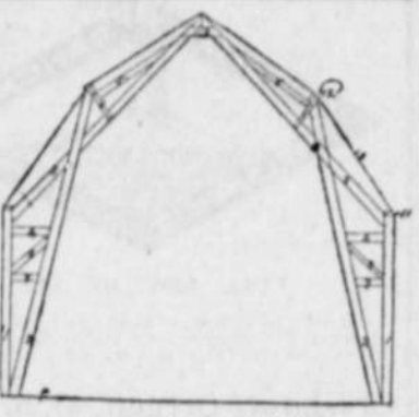
PLANK SYSTEM FRAME.
