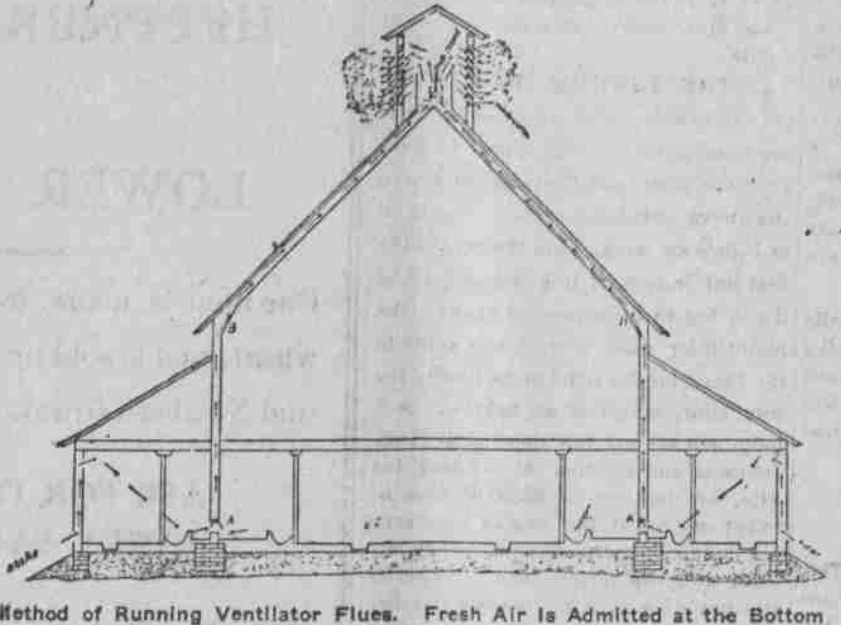
Method of Running Ventilator Flues. Fresh Air is Admitted at the Bottom and Foul Air Taken Out at A and B.
