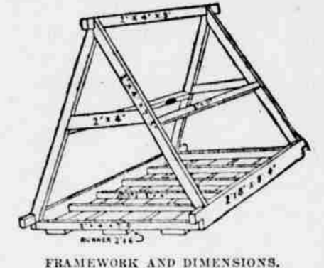
FRAMEWORK AND DIMENSIONS.
