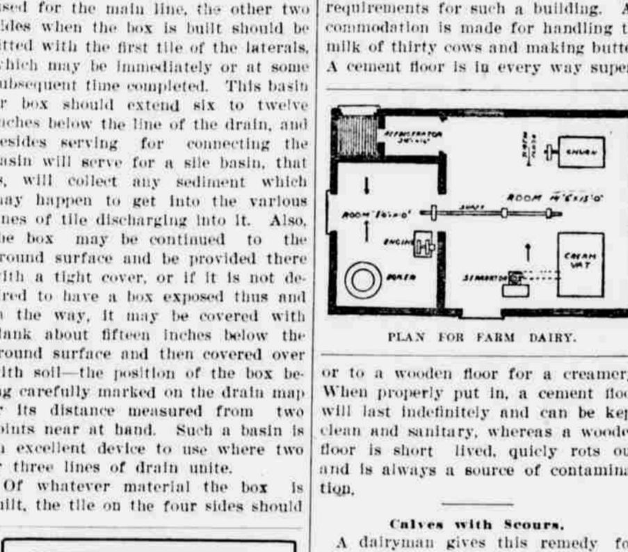
PLAN FOR FARM DAIRY.
