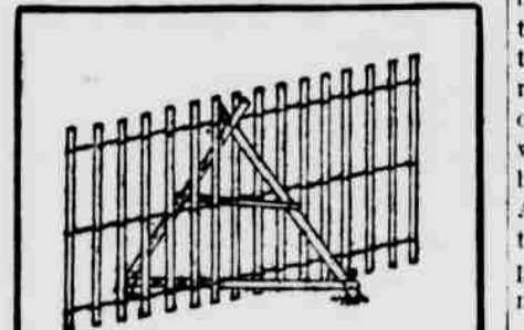
SUPPORTS FOR FENCE.
