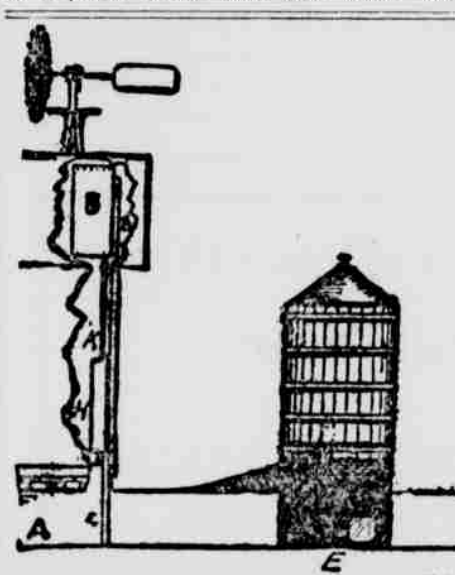
ARRANGEMENT FOR WATER SUPPLY.
