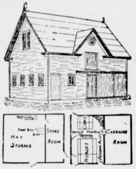
GOOD BARN PLAN.
