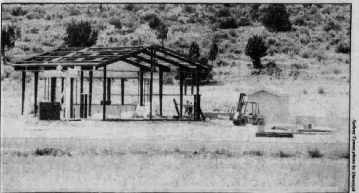
Part of the renovation project in Warm Springs includes the remodeling of the Old Administration Building and the construction of three new buildings to house offices and equipment for Bureau of Indian Affairs Roads department, Land Operations and Facilities Management departments. Buildings are expected to be completed by the end of January, 1988.
