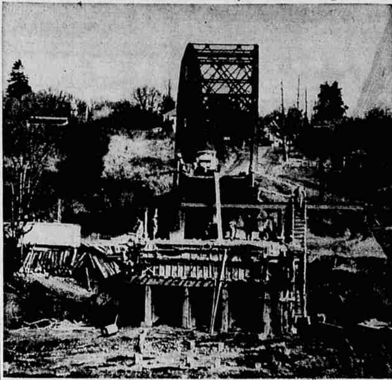
LAFAYETTE—Modern highway bridge replaces willow old horse and buggy structure spanning the Yamhill river on the road between Lafayette and Dayton. Completion date is set for Oct. 1. (Capital Journal Photo)
