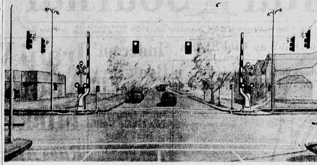
When a train approaches the intersection, it causes the traffic signal to change immediately to the all red indication in all directions. At the same time the flashing light portions of the railroad drop arm gates start to function.
