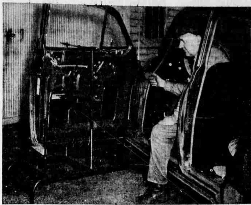
Harvey J. Burington, proprietor of the 12th Street Body and Paint shop, pointing out stand invented by him for supporting car doors while door is being aligned to hinges on body of the car.
