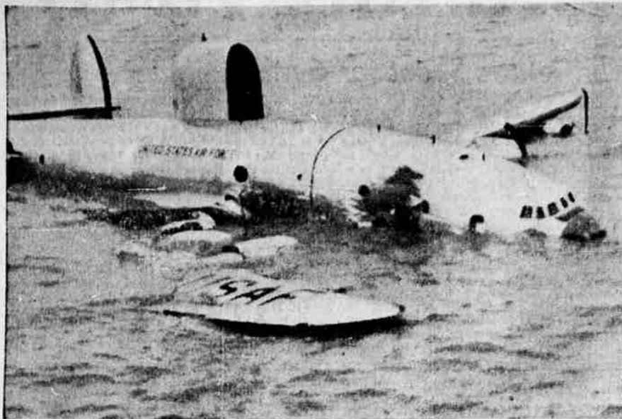
This four-engine Super Constellation lays in shallow water after crash-landing in a heavy fog while making a landing approach to Hamilton Air Force Base off San Francisco Bay.
