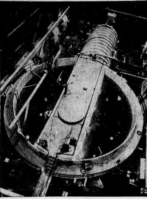
The first atomic submarine engine, built into a land based submarine hull, was generating power when this overhead view was made at the National Reactor Testing Station in Idaho. The engine section is immersed in a sea tank about 50 feet in diameter and almost 40 feet high to simulate actual operating conditions. The nuclear power plant, designed and built by Westinghouse Electric Corporation, is a prototype of the engine in the USS Nautilus, first atom submarine scheduled to be launched Jan. 21 at Groton, Conn. (AP Wirephoto)
