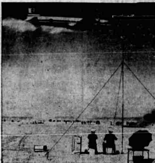
A four-engine transport plane dumps 1,600 gallons of water on simulated brush fire in test at Fossomond Dry Lake in Southern California, as officials watch. Fire fighting officials envision method as means of checking forest fires in rugged terrain until ground parties can reach the areas. Purpose of tests was to determine the pattern of water dispersal from the plane. (AP Wire-photo)
