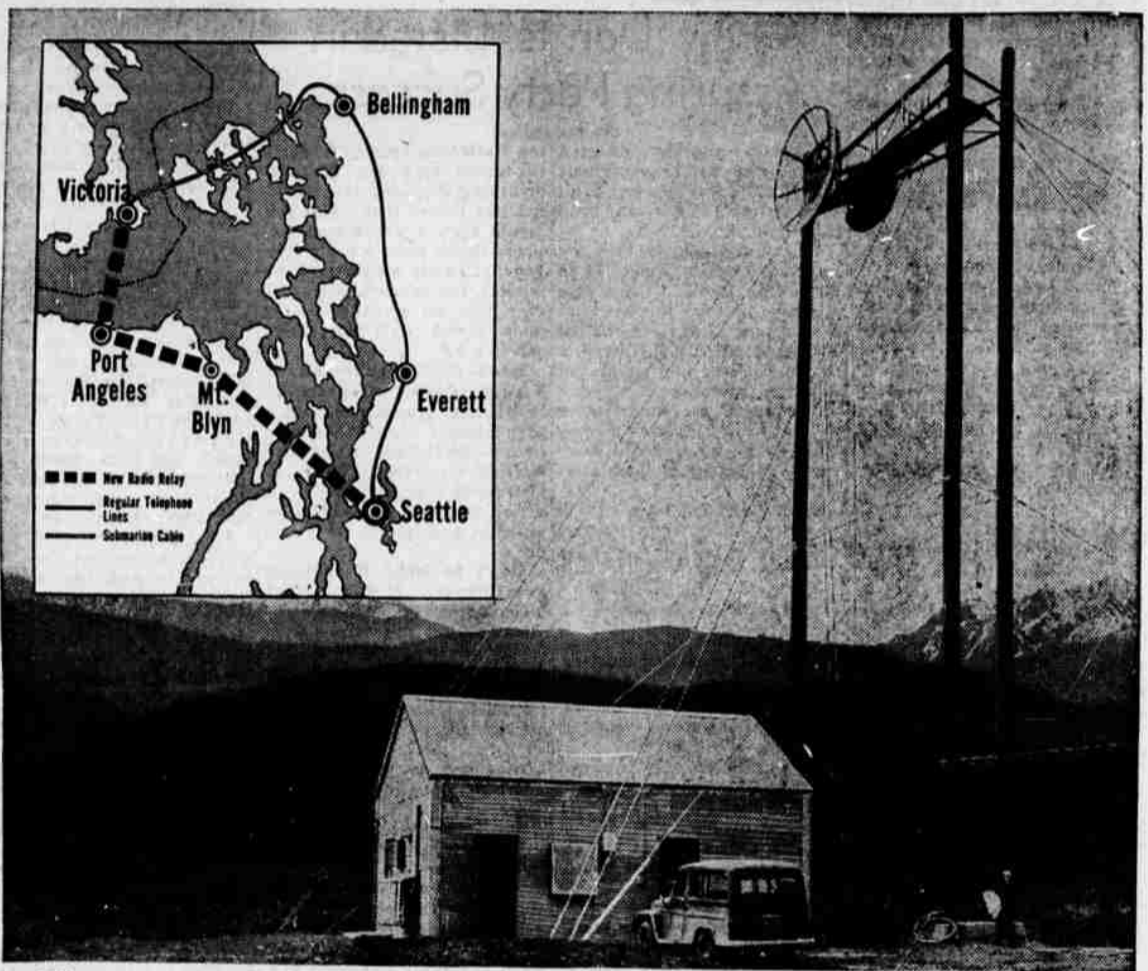
This tower atop Mount Blyn, Washington, is an intermediate station for telephone calls carried by radio-relay back and forth across the international border between Seattle and Victoria, B. C.
