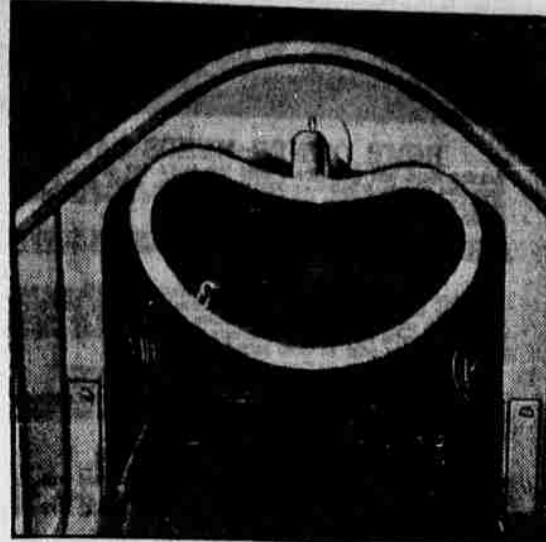
Remember, kids, the steering wheel for the 1953 Derby racer must be in a vertical, or near vertical position. Steering cables must be connected to the axle through pulleys and must have an adjusting turnbuckle somewhere along the cable.
