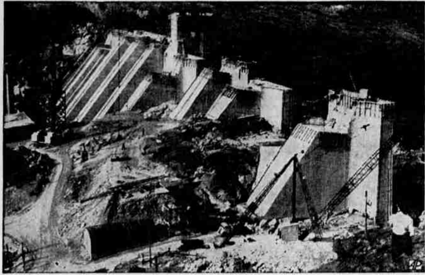
Power From the Highlands—Hydroelectric plant dam being built at Loch Sloy, Scotland, 788 feet above sea level where more than 100 inches of rain falls annually.
