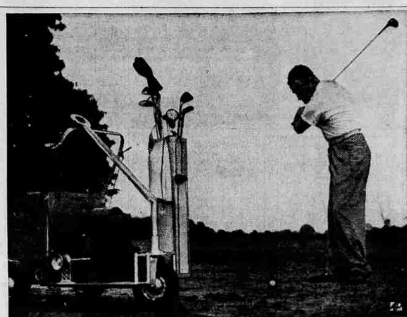
Links Chariot Lou Billinger, Indianapolis, rides this cart chariot—style between strokes of a round of golf. It carries him over the course at from 2 to 4 miles an hour.
