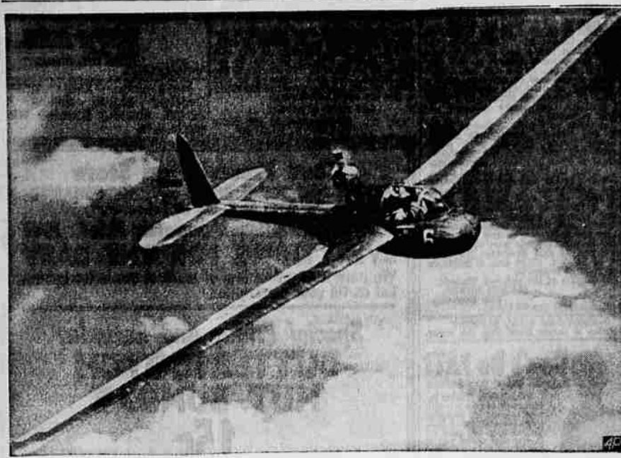
Glider Aided by Outboard Motor—This sailplane in flight over the Arlington State college airport at Grand Prairie, Tex., uses an auxiliary motor, visible back of cockpit, to get into the air instead of the conventional tow rope. Motor folds forward into the plane's body after ship gains enough altitude to soar. Ted Nelson of Oakland, Calif., builder of the plane is at controls. (AP Wirephoto)
