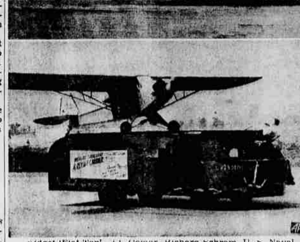
Midget 'Fiat Top'—Lt. Comdr. Richard Schram, U. S. Naval Reserve pilot, gets set to come in for landing on a truck with a 17-foot deck built atop at Northerly Island, Chicago. Plane settles down (lower photo), and holds position as truck comes to a halt. The small cabin plane also takes off from the midget deck. Stunt was rehearsed for an air show at the U. S. naval station in Glenview, Ill. (AP Wirephoto)
