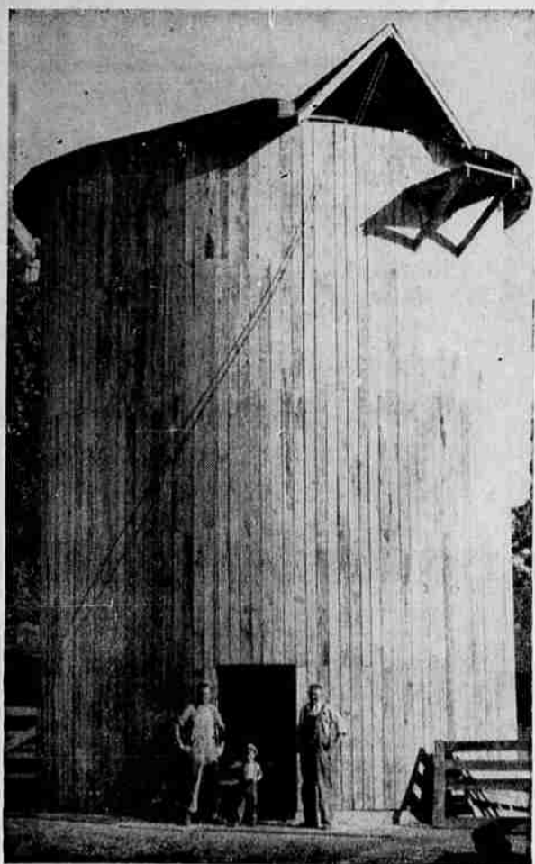
Dallas—First of its type in Polk county, a new hay storage barn and dryer at the Chester Jenkins' farm, Greenwood, will hold between 50 and 60 tons of hay and can be constructed at a cost of about $1000. The circular shed has a shaft running vertically through the center as an air vent. A blower may be placed in the doorway at the bottom to force air up the shaft and through the hay. Cracks are intentionally left between the exterior sheathing to allow an exit for air. In the picture are Marvin Jenkins (left), father of Fred Jenkins (center) and son of Chester Jenkins (right). The shed now nears completion and will be filled soon with chopped hay. (Abel photo)
