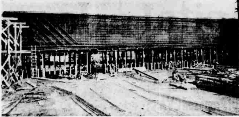
Salem's Largest Beam—Reinforced concrete beam, now being poured by L. H. Hoffman, contractor for the Capitol street shopping center, is 116 feet long, 15 high and 13 inches thick. This massive beam that carries the roof and front of the building required 265,400 pounds of concrete and 13 1/2 tons of steel. Use of this construction eliminates need for center posts.
