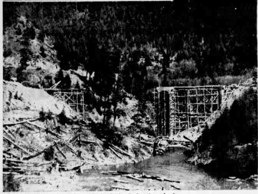
New Highway Bridge Spans Breitenbush —Re-location of North Santiam highway above the reservoir of Detroit dam required construction of this reinforced concrete, steel girder type bridge 440 feet in length. This structure and a shorter bridge over Tumble Creek are being constructed by the Port Construction company of Portland under supervision of the Federal Bureau of Roads.
