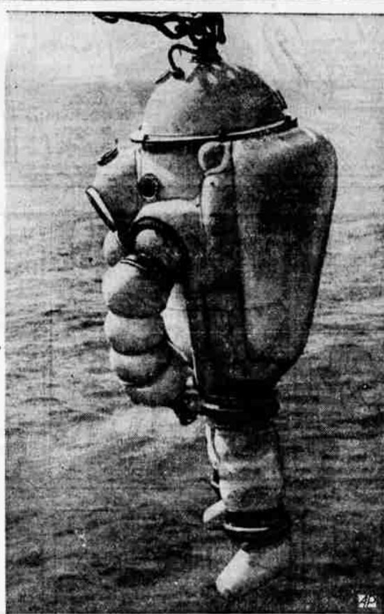
NOT 'DOPEY,' THE DWARF, this is a new diving apparatus at La Spezia on the west coast of Italy by G. Galeazzi, who's giving it tests in the Gulf of Genoa. The diving apparatus, which weighs almost 900 pounds, went down to a depth of about 800 feet on its preliminary trials at La Spezia.
