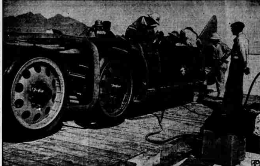
Mechanics Check Gears in Race Car—Inability to shift gears easily caused George E. T. Eyston, British race driver, trouble in his early test runs at Bonneville Salt Flats, Utah, where he hopes to establish a new world's auto speed record. Mechanics are shown removing the machine's streamlined sides preparatory to working on the gears. Captain Eyston (wearing cap, hands behind back) watches the work progress. (Associated Press Photo.)
