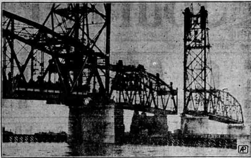
Towed ten miles, a 303 foot portion of the San Mateo bridge across San Francisco bay was fitted to adjoining spans as the tide went out. The structure is 7.1 miles long.
